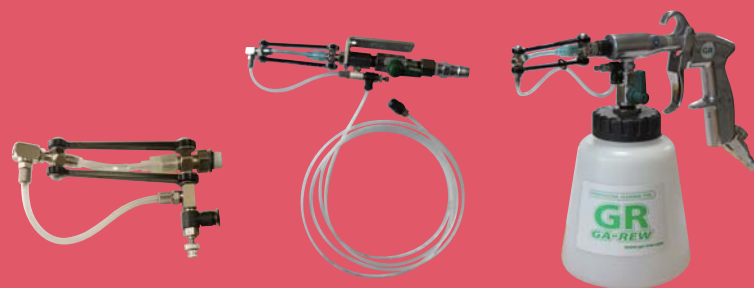
Nozzle Unit
