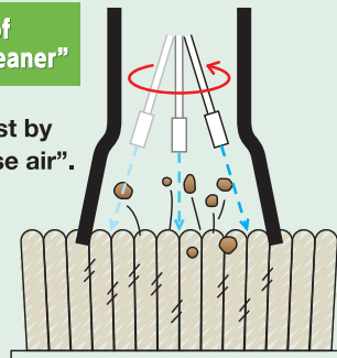
"Internal view of Tornado Vacuum Cleaner"
